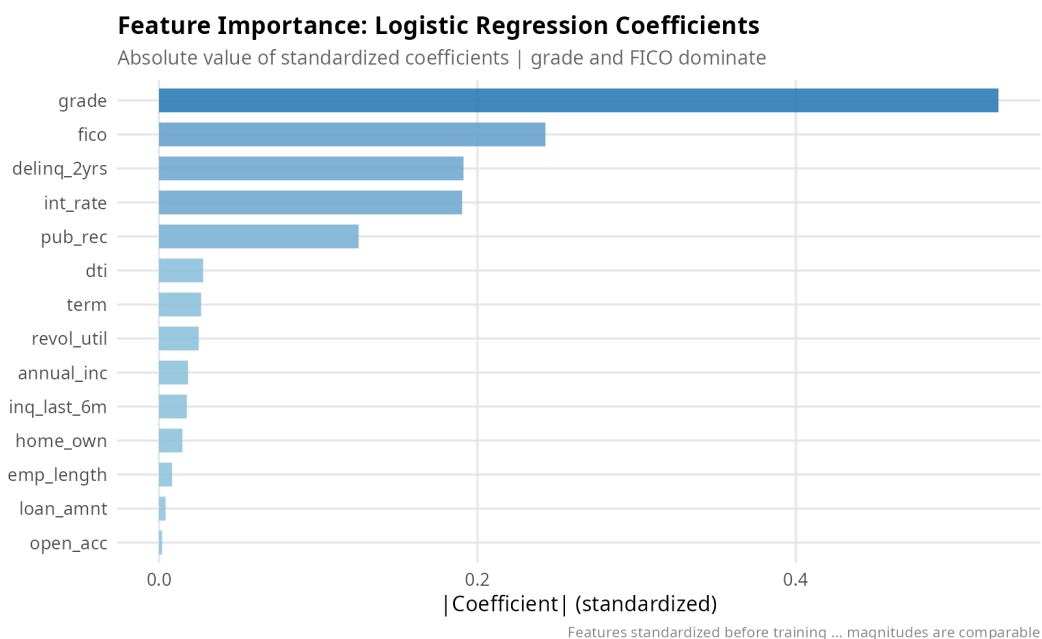
Figure 7. Logistic regression coefficient magnitudes on standardized features. grade and fico dominate; delinquency history and interest rate follow.
