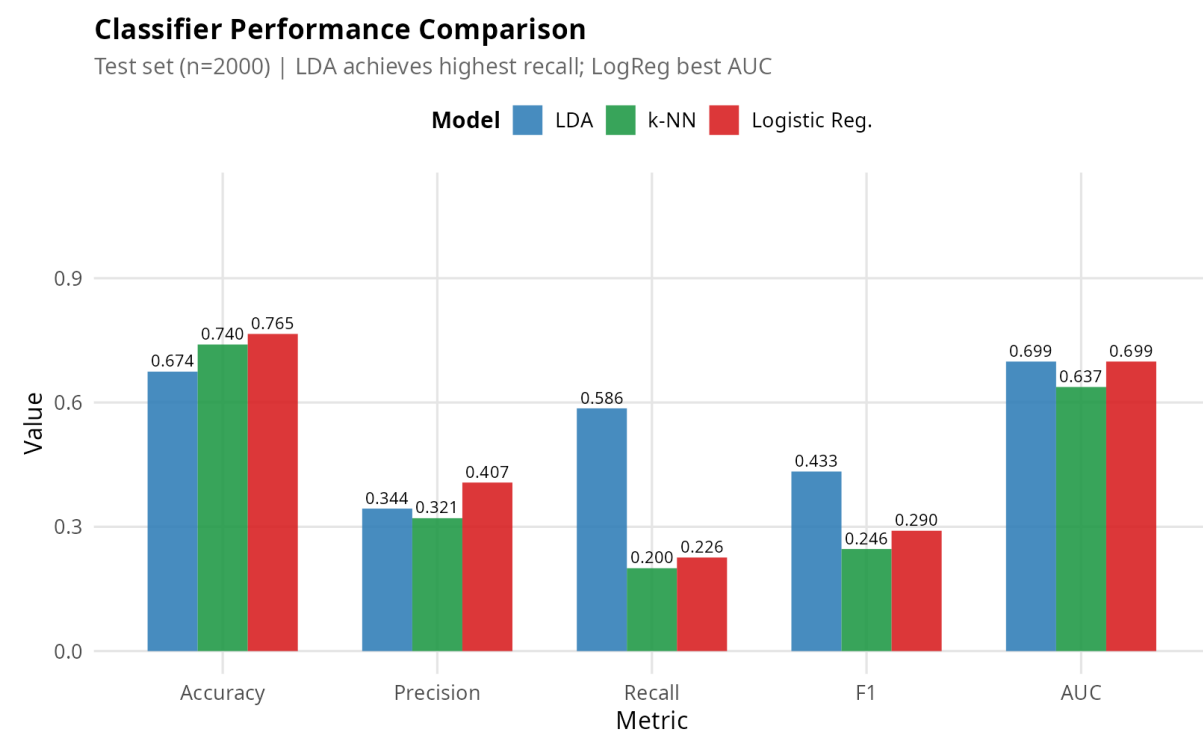
Figure 6. Classifier metrics on the test set ( n = 2,000 ). All metrics computed at each model's chosen decision threshold.
