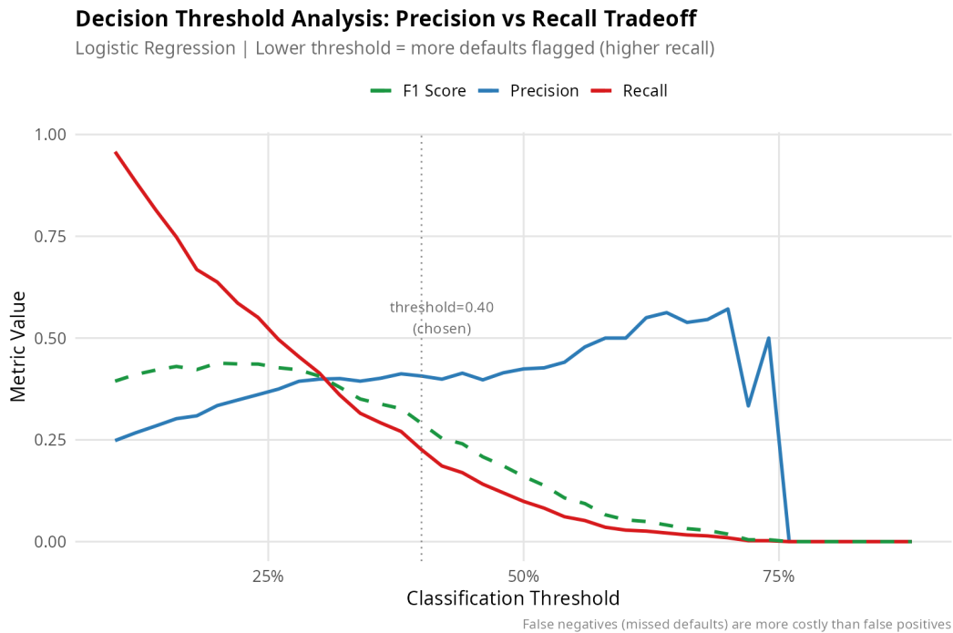
Figure 8. Precision–recall tradeoff as a function of decision threshold for Logistic Regression. A threshold of 0.40 (rather than 0.50) is chosen to increase recall at the cost of some precision.
