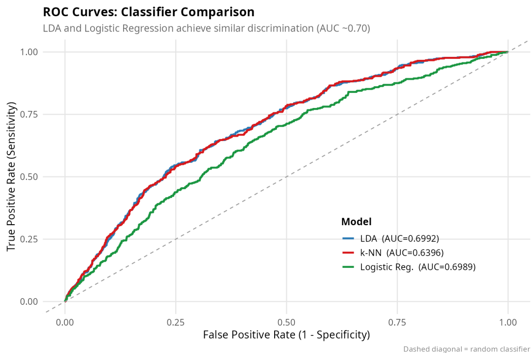
Figure 5. ROC curves for all three classifiers. LDA and Logistic Regression achieve AUC \approx 0.70 ; k -NN underperforms due to the curse of dimensionality in 14-dimensional feature space.
